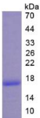
Figure 1. SDS-PAGE
