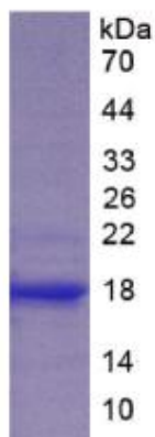
Figure 1. SDS-PAGE
